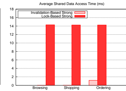
Fig. 5. Average time (ms) to access a shared data table.
