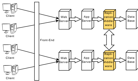
Fig. 1. Replication model.
