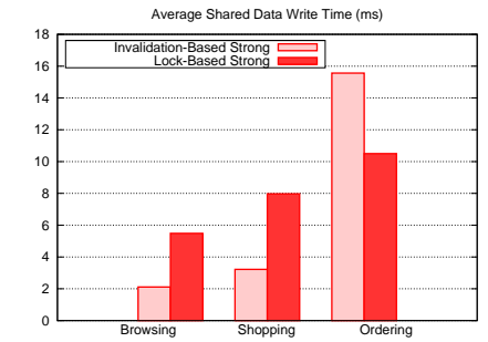
Fig. 6. Average time (ms) to write to a shared data table.
