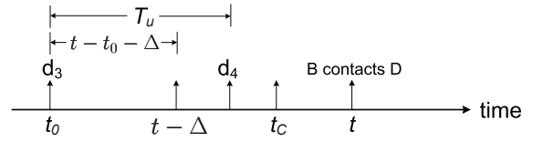
Fig. 7. Calculating the utility of data updates
