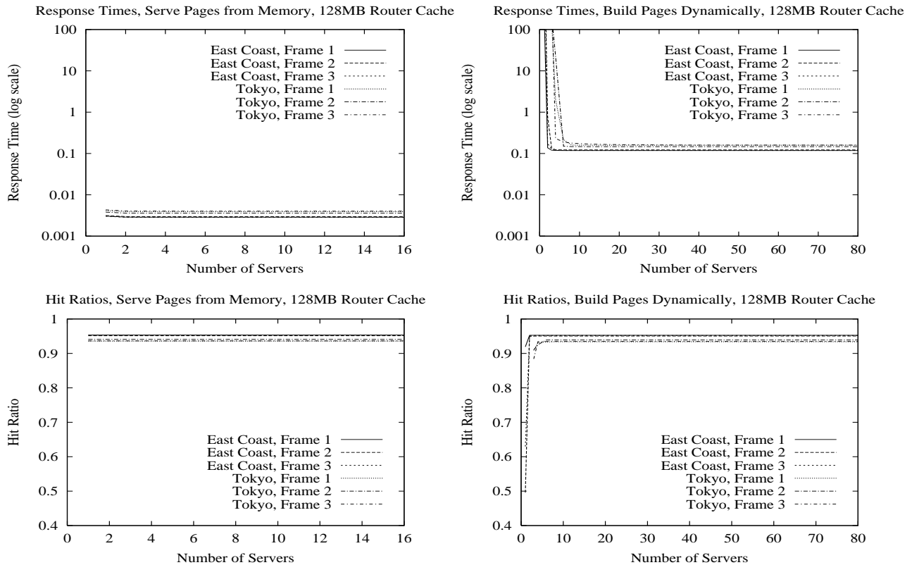
Fig. 9. Mean response times and cache hit ratios for 3 representative SP2 frames from the East Coast and Tokyo sites, each with a POD cache farm.
