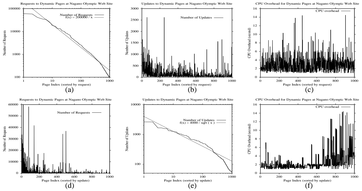
Fig. 5. Request and update distributions to dynamic pages
