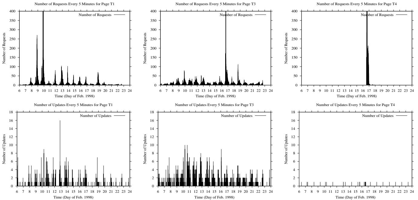
Fig. 6. Requests and updates to the 1st (T1), 3rd (T3) and 4th (T4) most popular dynamic pages from Asia
