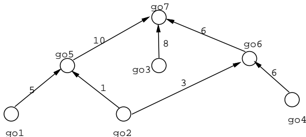
Fig. 1. An object dependence graph. Weights are correlated with the importance of data dependencies.
