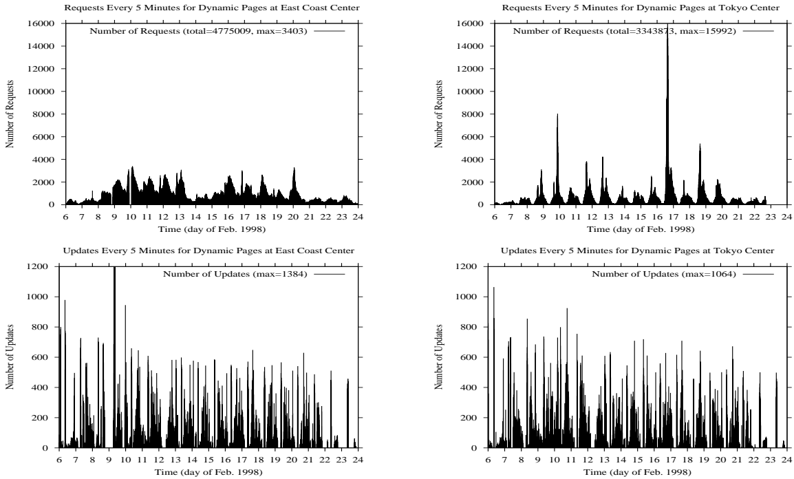
Fig. 4. Request and update patterns every 5 minutes at the East Coast and Tokyo sites
