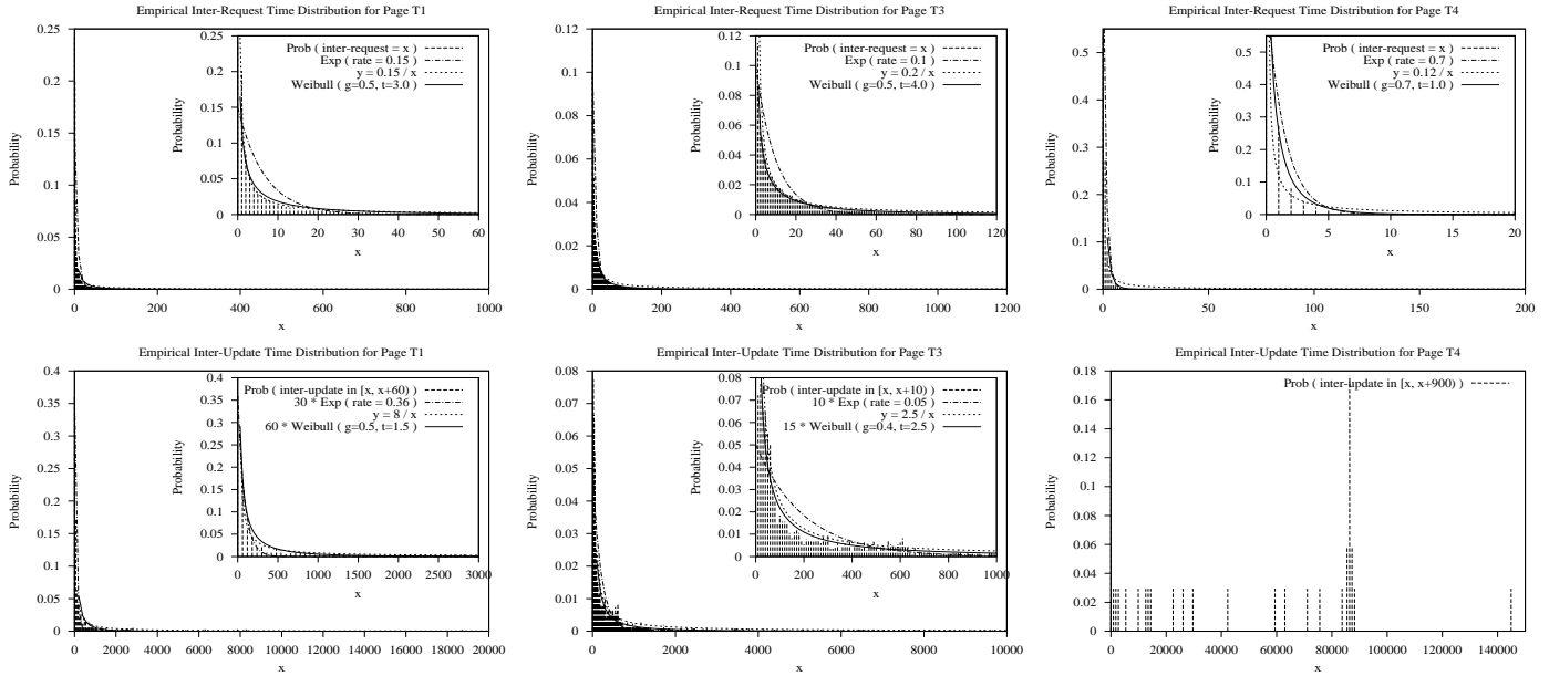
Fig. 7. Interrequest and interupdates times for the 1st (T1), 3rd (T3) and 4th (T4) most popular dynamic pages from Asia
